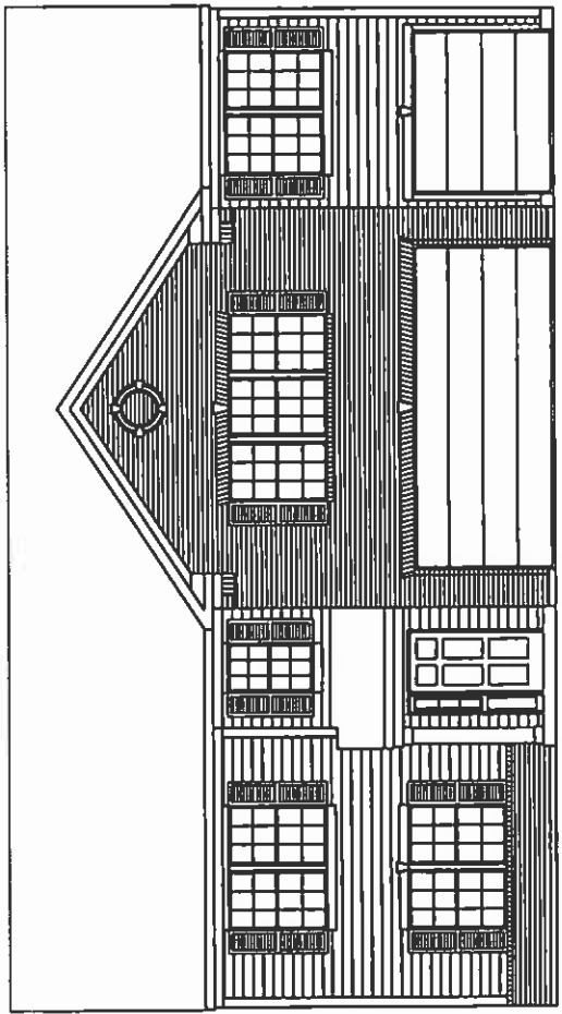
FRONT ELEVATION A
